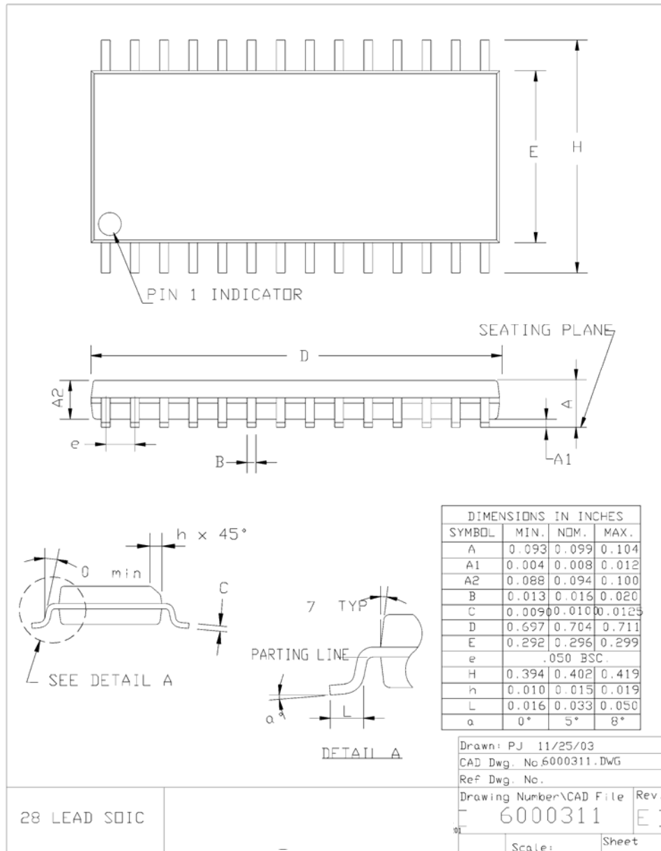
Figure 8: Package Outline Drawing
