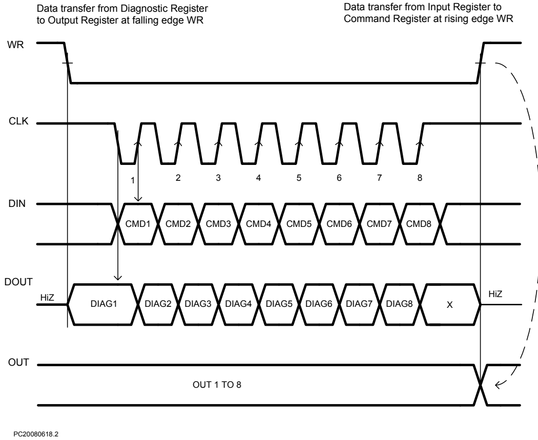
Figure 7: Timing Diagram
